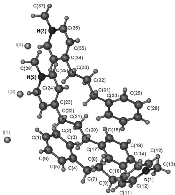
Figure 2. The crystal structure of [(\text{C}_6\text{H}_5)(\text{CH}_2)_3(\text{C}_5\text{H}_4\text{N}(\text{CH}_3))]^+\text{I}^- 1 showing the three units with atomic numbering scheme. The two halves of the pyridine ring (N(1), C(10)–C(12)) are related by the symmetry operation x, 1.5-y, z , and all the other halves of the rings by the symmetry operation x, 0.5-y, z .
