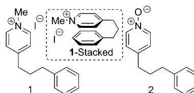
Figure 1. Phenylalkylpyridine derivatives 1 and 2 .
