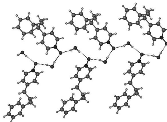
Figure 5. The crystal packing of 2.H 2 O showing hydrogen bonding along the a axis.
