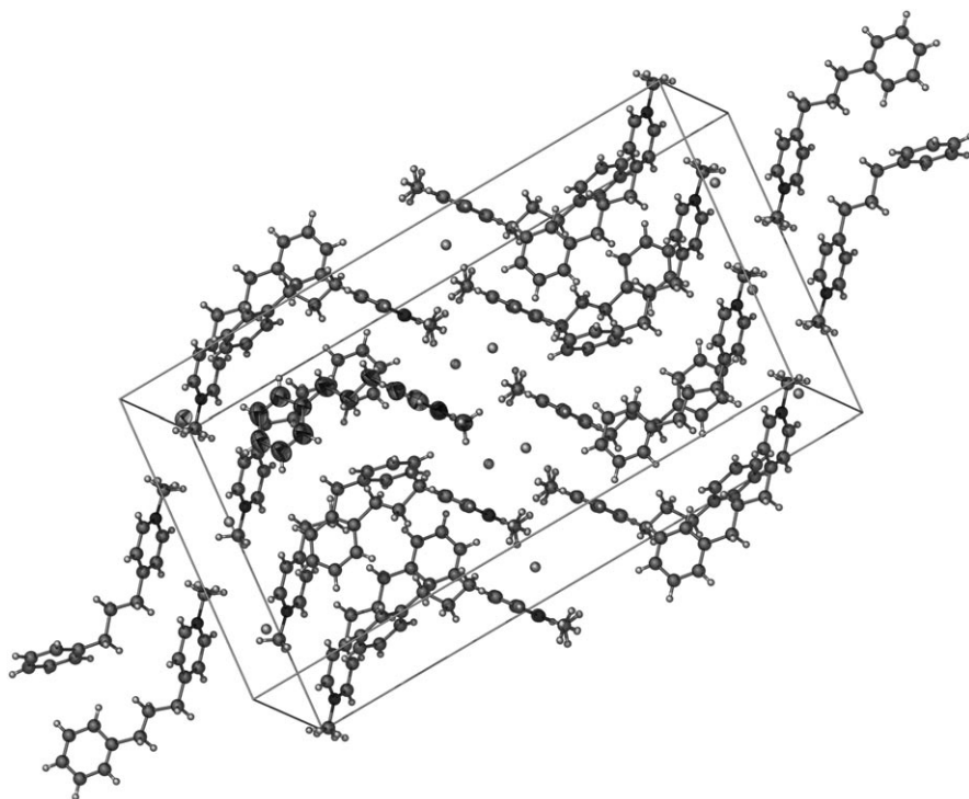
Figure 3. Crystal packing of 1 showing the channels of I^- ions running parallel to the c axis.
