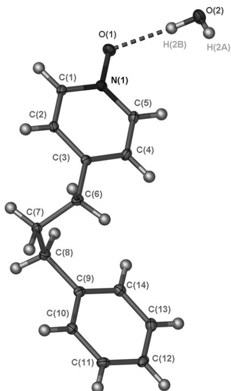
Figure 4. Crystal structure of one unit of [(C_6H_5)(CH_2)_3(C_5H_4N^+O^-)]H_2O 2 . Anisotropic displacement parameters have been drawn at the 50% probability level and atom numbering scheme is also shown.
