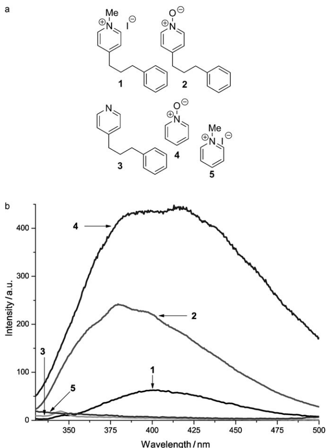
Figure 6. a) Compounds compared by Fluorescence Spectroscopy. b) Emission spectra of compounds 1–5 , 1 \times 10^{-4} M (CH 2 Cl 2 ), excitation at 315 nm.
